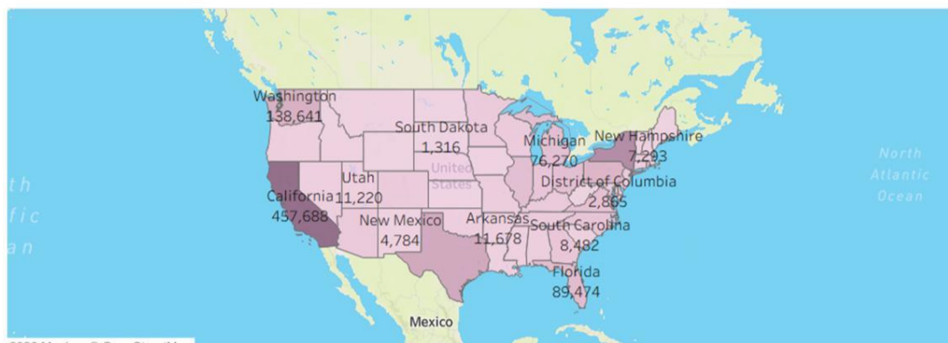
Map Chart
