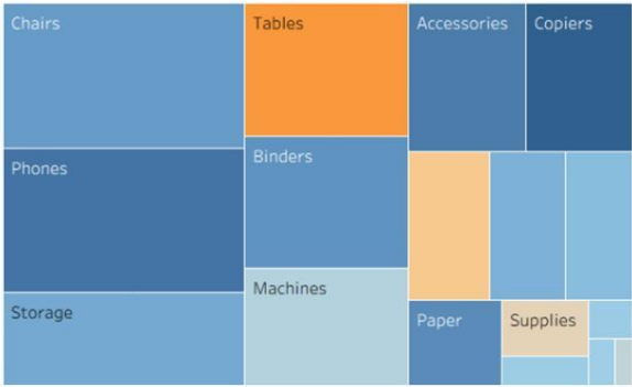
Tree Map
